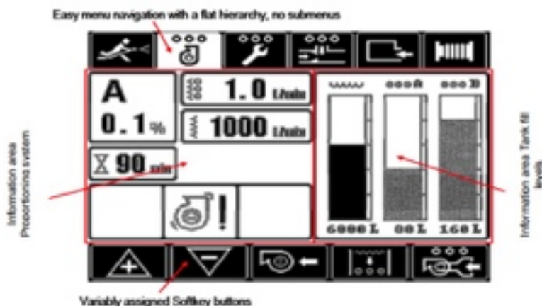
Figure 03: Information display of the HMI control unit, options coloured
